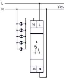
Direct control of the emergency light systems 1 ≤ ⚡ Emergency light systems with own battery sup.
