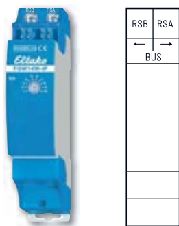
Function rotary switch
