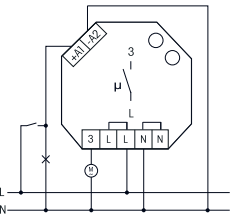
Fan control through light switch
