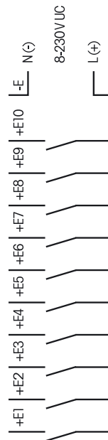
Control inputs FTS14EM
