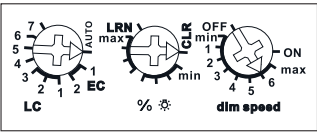
Function rotary switches on the side
