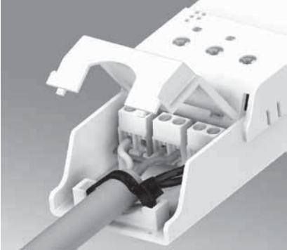
The cable must be fastened with standard cable ties (width <3,6 mm).
