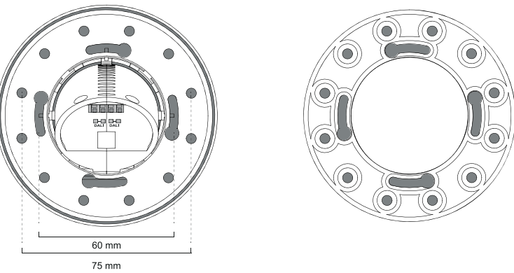
Dimensions of mounting ring
