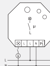
Typical connection
