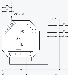
4-wire circuit with attic lighting, resettable
