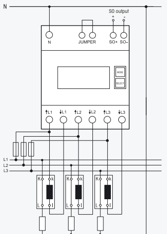
Typical connection 4-wire-connection 3x230/400V
