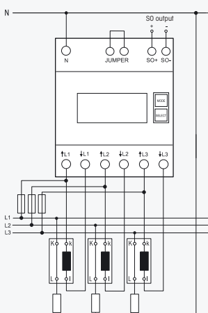
Typical connection 4-wire-connection 3x230/400V
